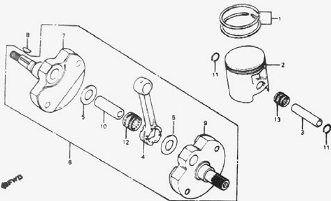
CR250R '81 - '82 - '83 Selection table of connecting rod large end bearing
